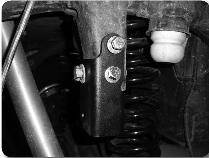
Figure 10 - LHD Shown
